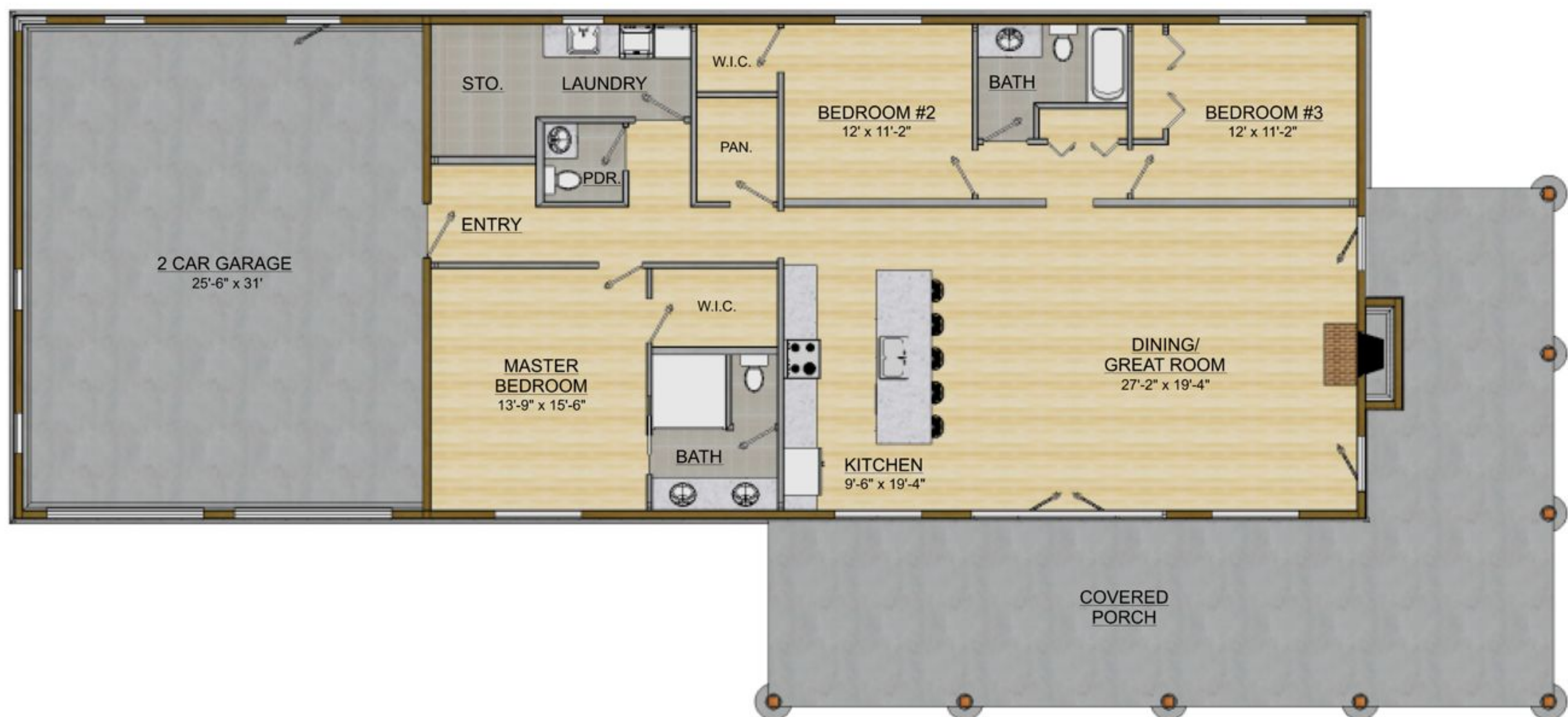
MAIN FLOOR PLAN
