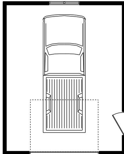
FLOOR PLAN 16'x20', 320 SQ. FT. FLOOR AREA
