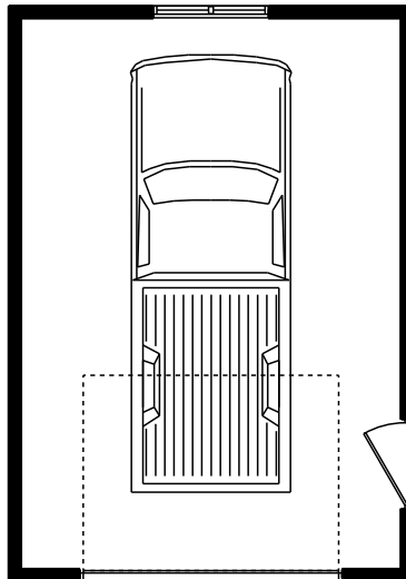
FLOOR PLAN 12'x20', 240 SQ. FT. FLOOR AREA
