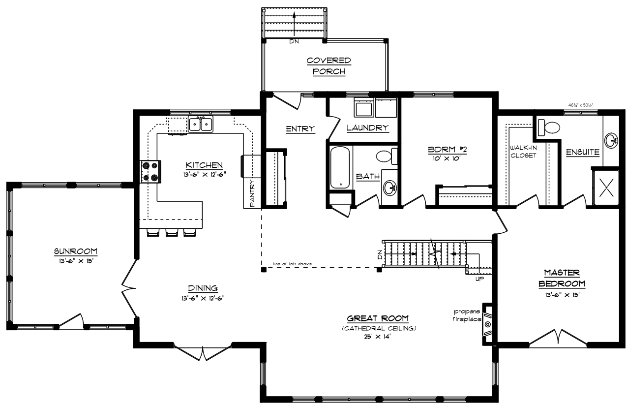
MAIN FLOOR PLAN 1860 SQ FT
