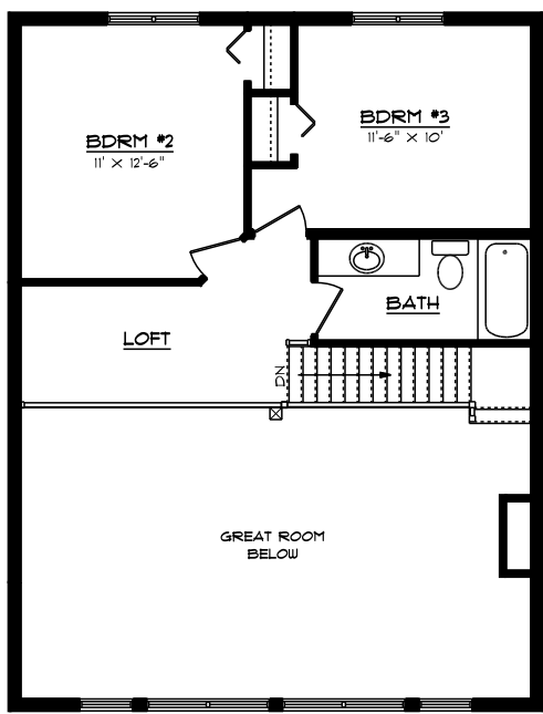
LOFT FLOOR PLAN 494 SQ FT
